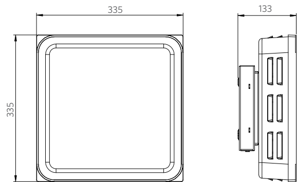
Recessed mounting
