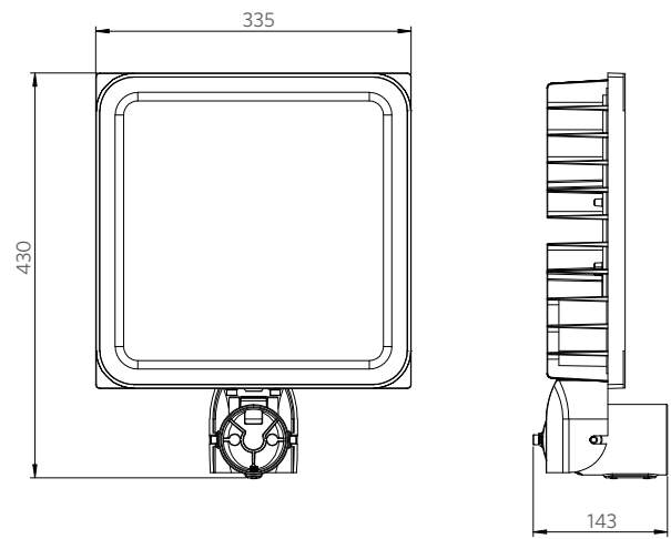
Pole mounting
