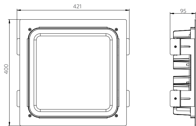
Recessed mounting
